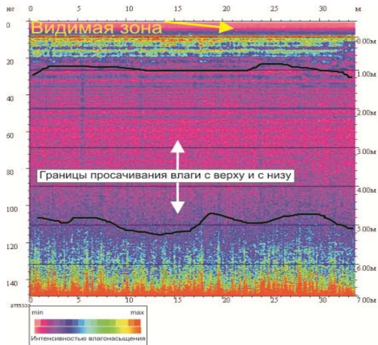
Picture 2 – An example of saturation zones isolation moisture in the dam body 1 according data GPR-sensing
