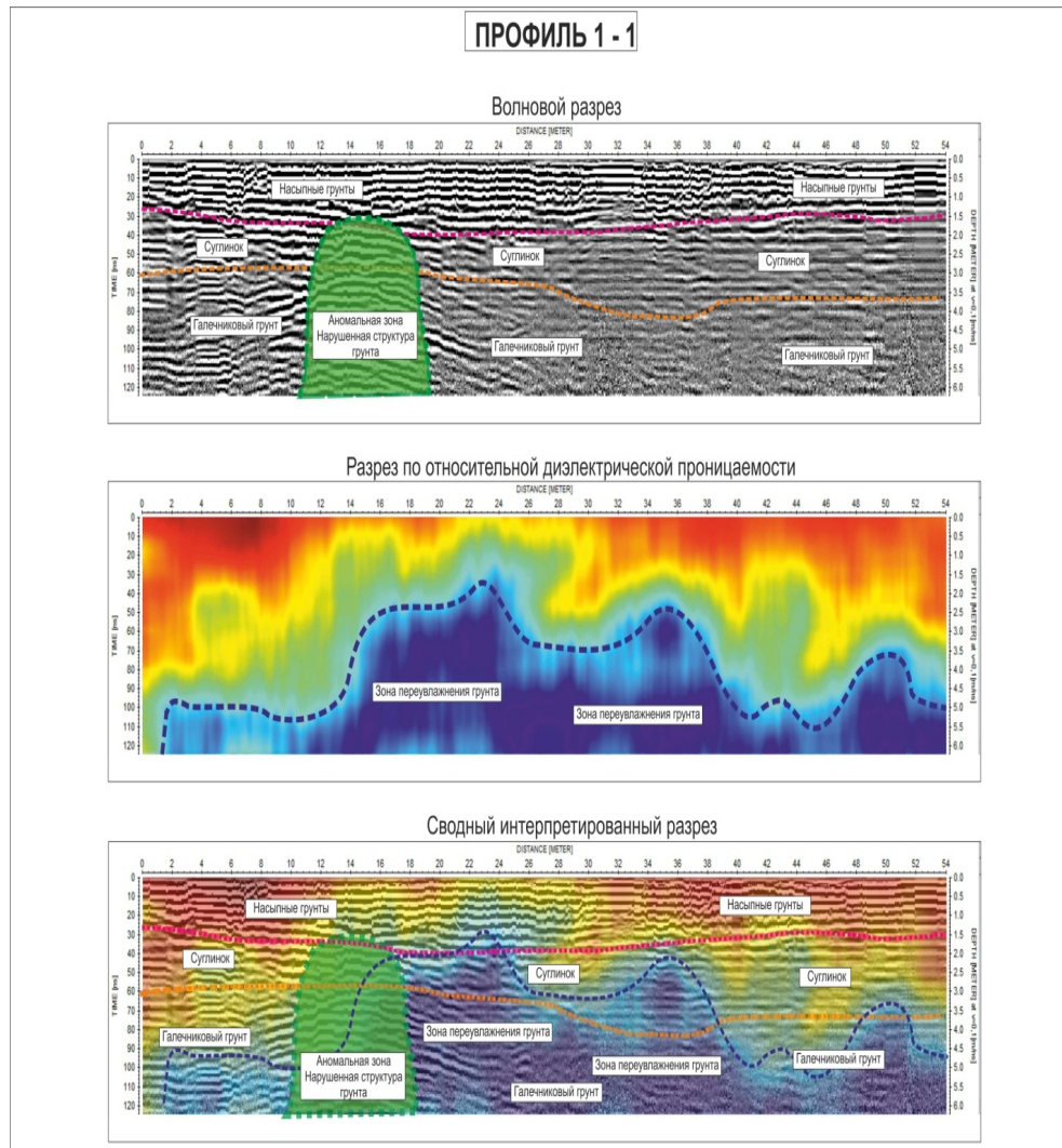
Picture 15 – The processed profile of the GRL behind the first retaining wall
