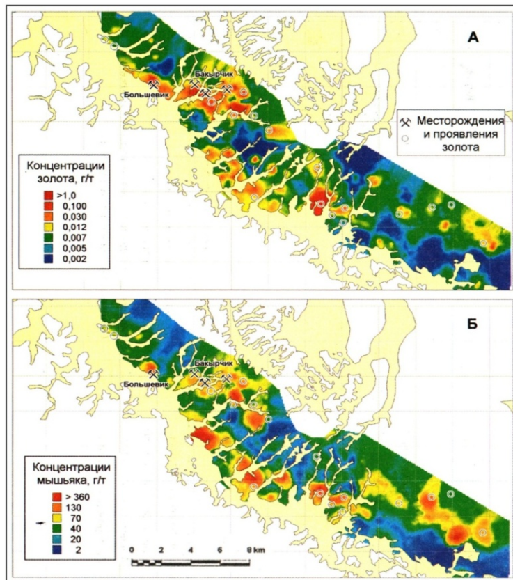
Figure 3 – Distribution of gold (A) and arsenic (B) in the area of the Kyzylovsky crushing zone (the Bakyrchik and Bolshevik deposits), based on the results of chemical testing [13]
