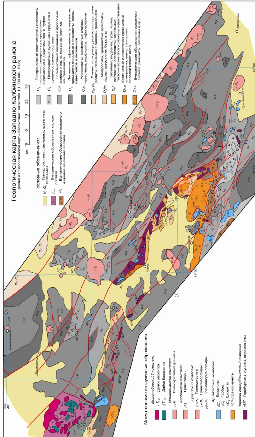
Figure 1 – Geological map of the West Kalba gold belt
