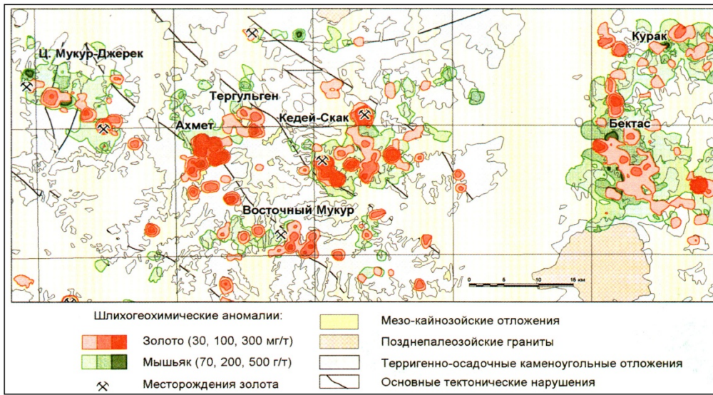
Figure 2 – Anomalies of gold and arsenic, identified by geochemical testing (Mukur-Bektas anomalous zone) [13]
