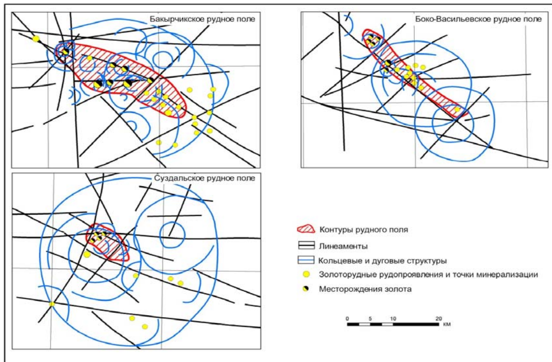
Figure 5 – Cosmo-structural models of ore fields [17]
