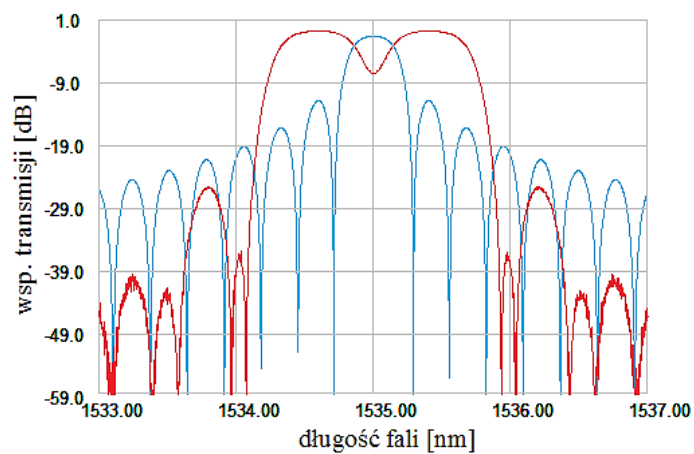
Figure 16 – Comparison of Bragg fiber gratings spectral characteristics without apodization – blue line and apodized Blackman function wsp. a = 5 – red line
