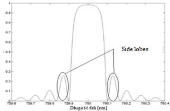
Figure 4 – Reflection spectrum of Bragg fiber grating
