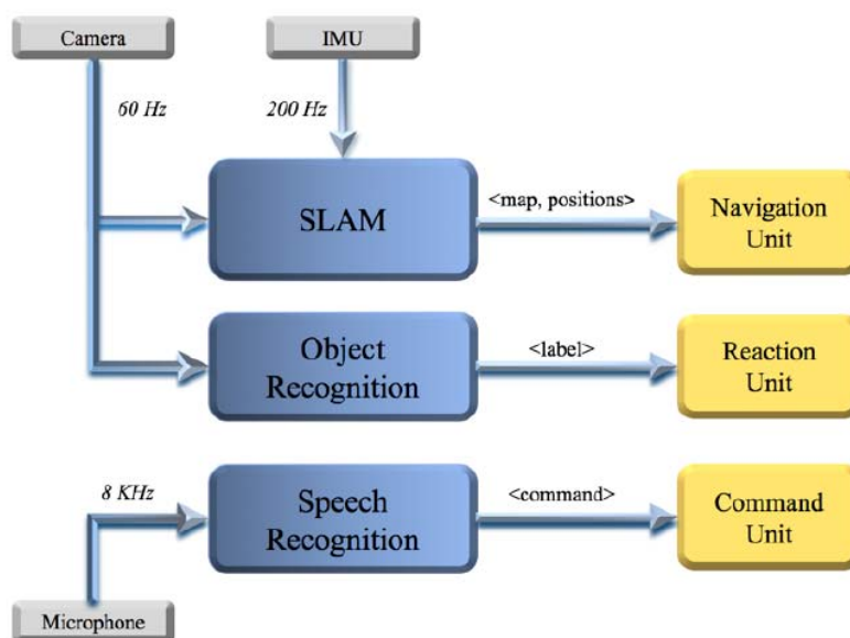
Figure 7 – System integration
