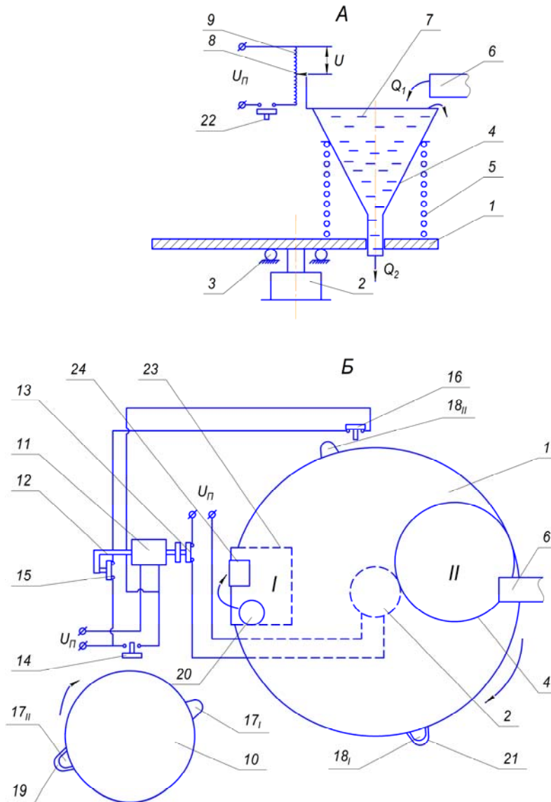
Figure 1 – The appliance for drilling mud density automatic monitoring.
