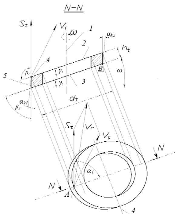
Figure 1 – Scheme for determining the working angles of a cutting tooth of a drilling tool
